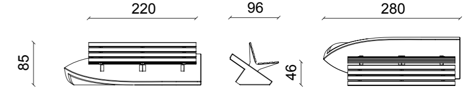
Panchina inclinata Panchina inclinata
