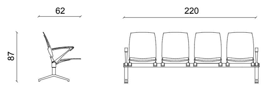
Panchina Delay 4 posti Panchina Delay 4 posti
